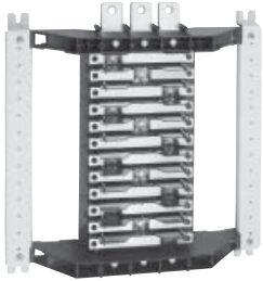
EasyPact™ Busbar EZB250W08
