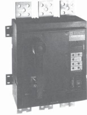
Sensor sizes : 1200-2500 A (PX, PE) 600-2500 ampere rating
